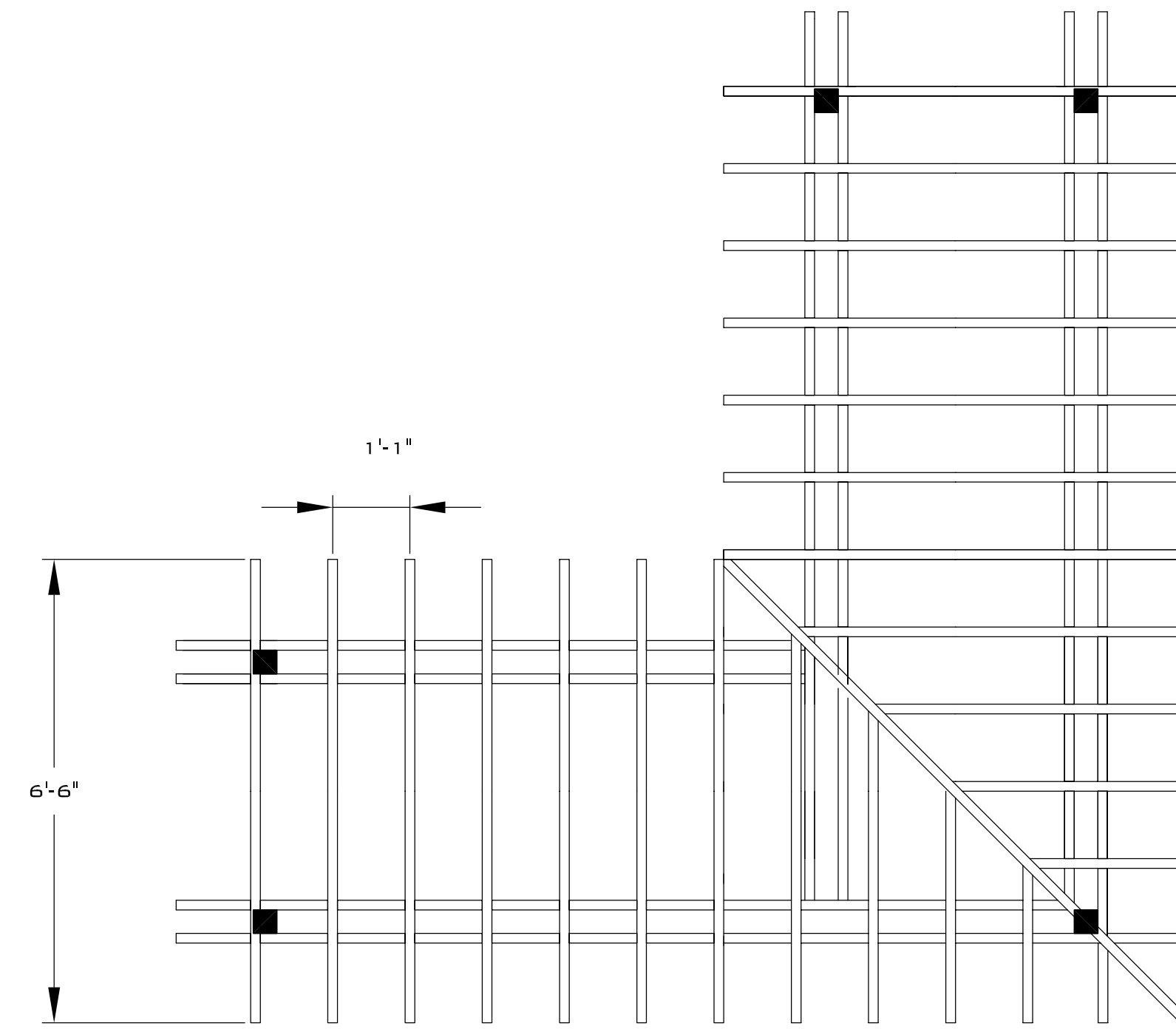
ARBOUR WITH OVERHEAD TRELLIS PIECES
