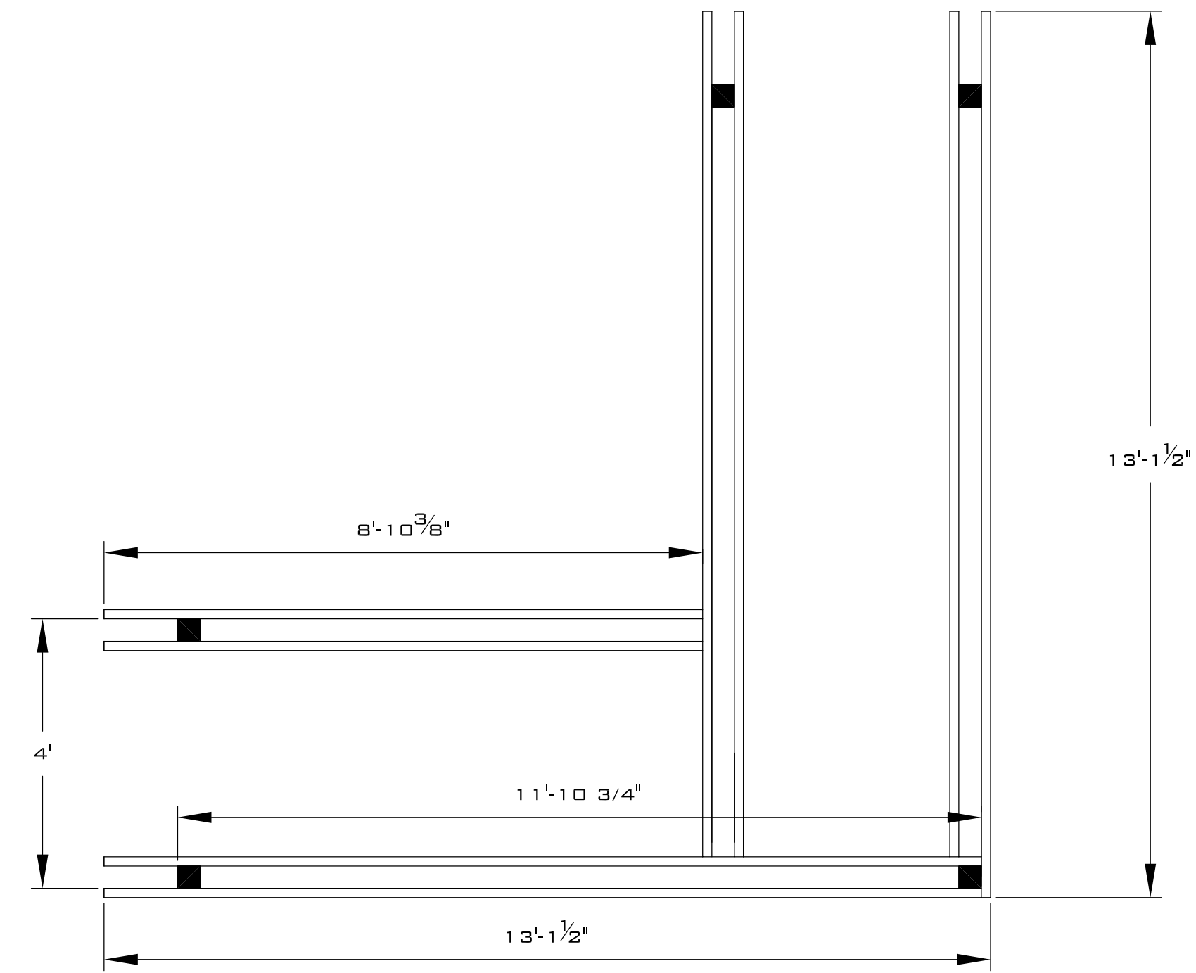
ARBOUR WITH OVERHEAD TRELLIS PIECES
